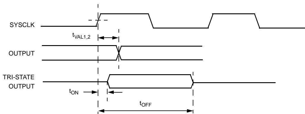
Figure 6-8. Output Timing
