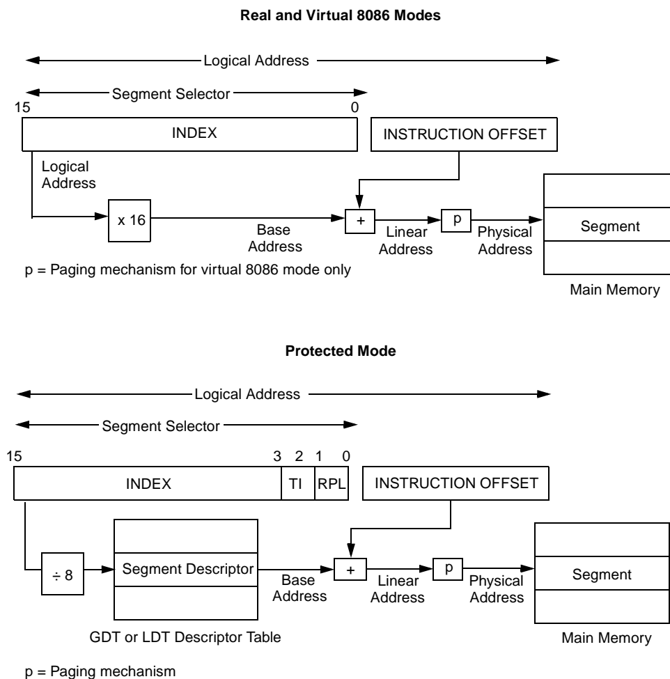
Figure 3-6. Selector Mechanisms
