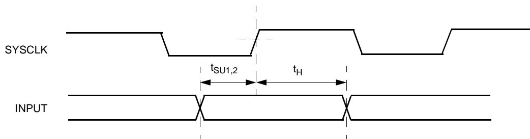
Figure 6-9. Input Timing
