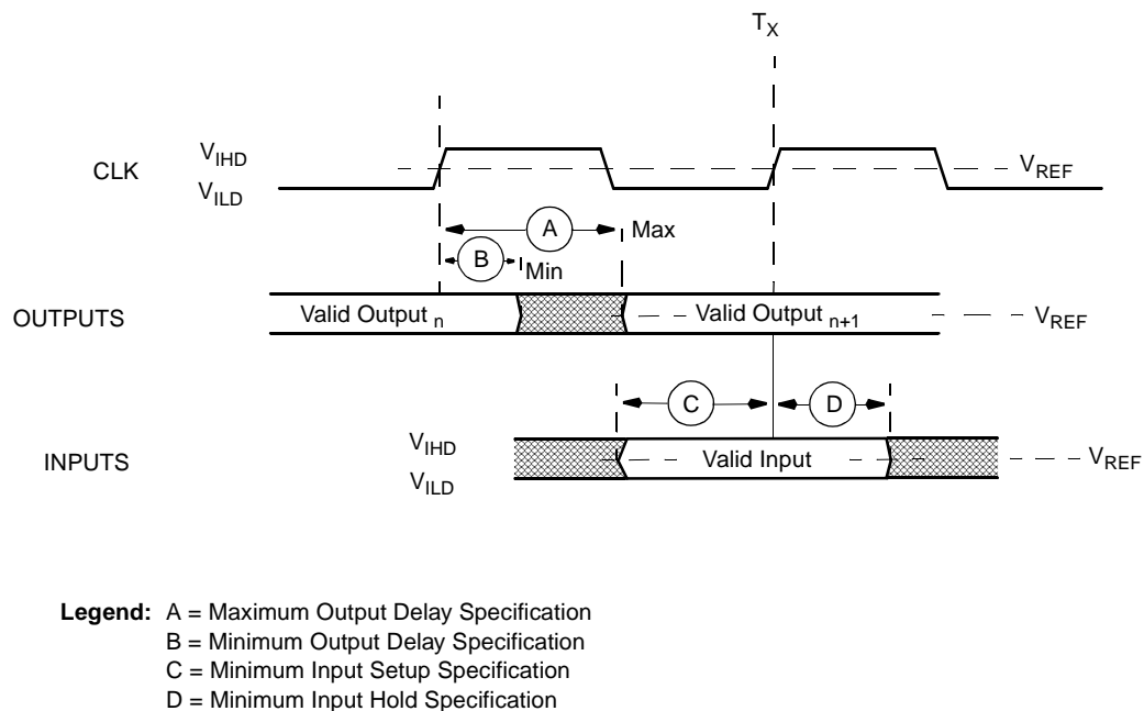
Figure 6-4. Drive Level and Measurement Points for Switching Characteristics
