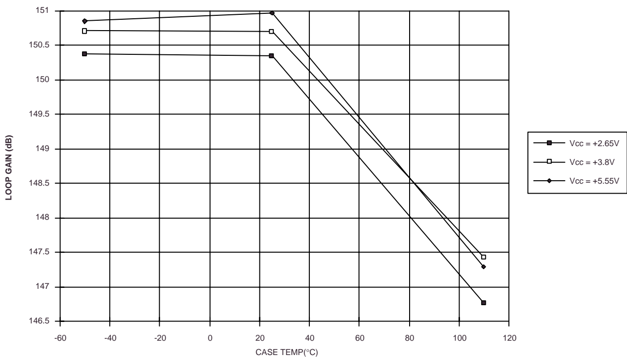
Fig. 13 On-chip Phase-locked-loop Synthesiser Loop gain
