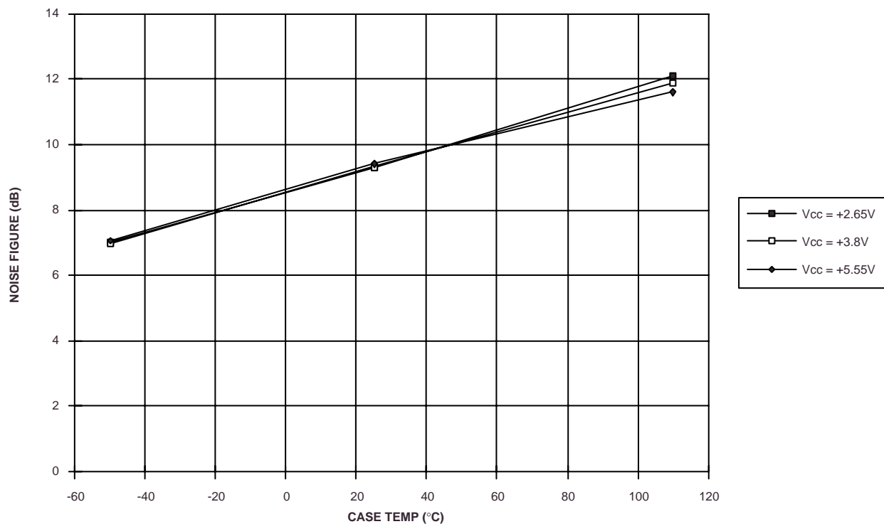
Fig. 12 Noise figure of IF chain in a typical application circuit
