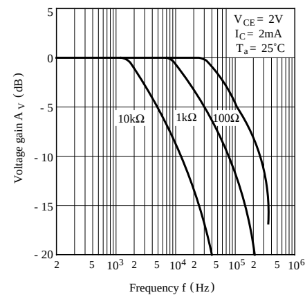
Fig.10 Frequency Response
