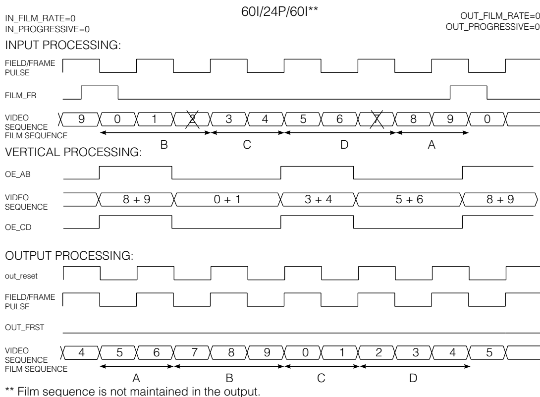
Fig. 22 60I/24/60I Processing
