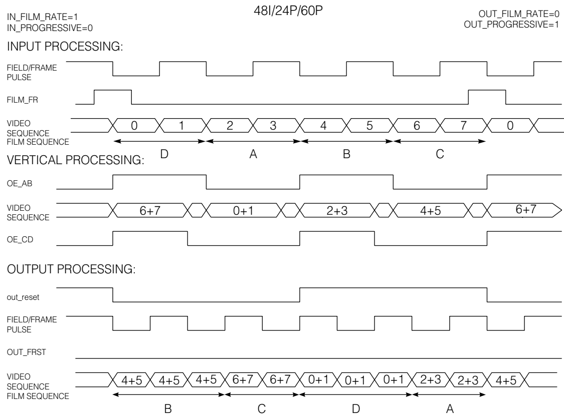
Fig. 33 48I/24P/60P Processing
