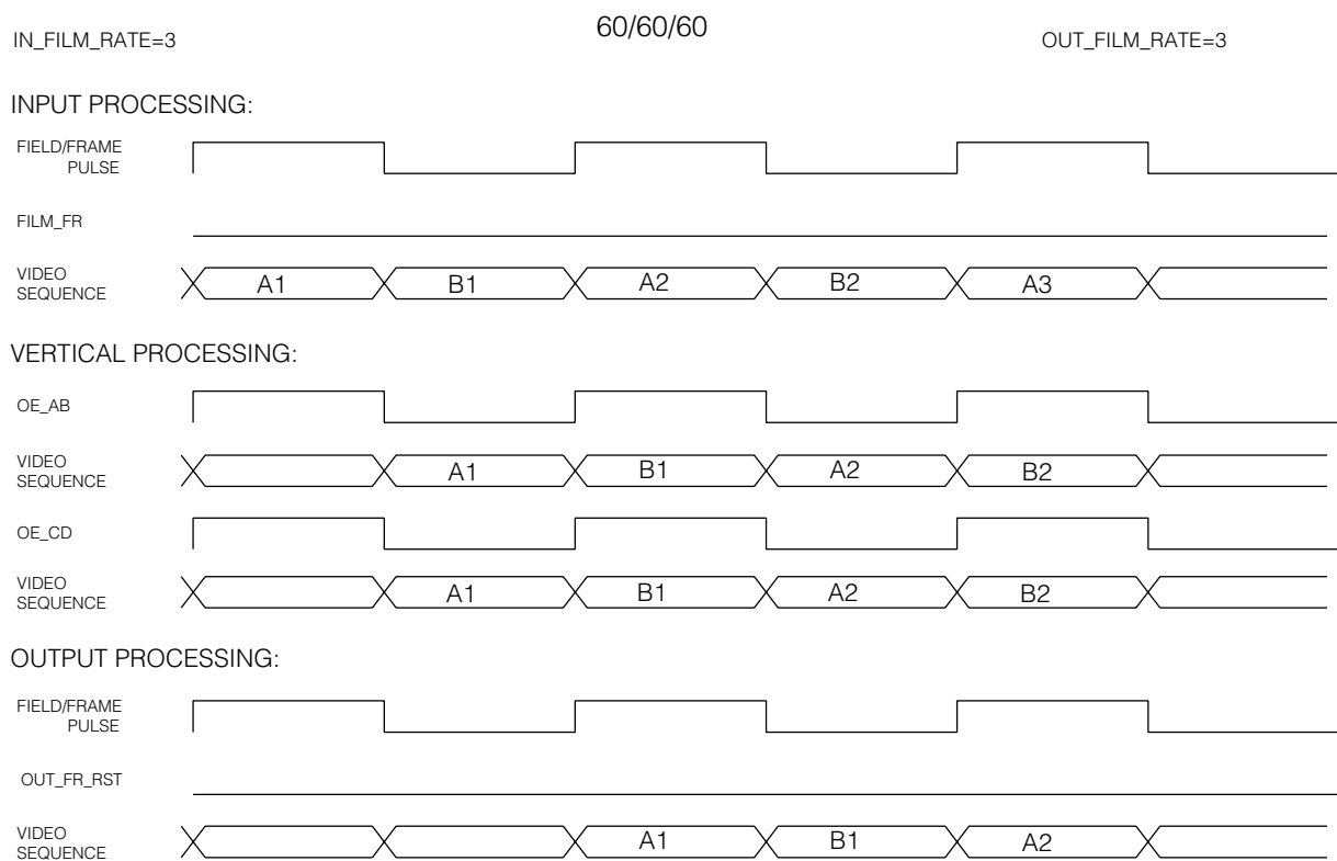
Fig. 17 60/6060/ Processing
