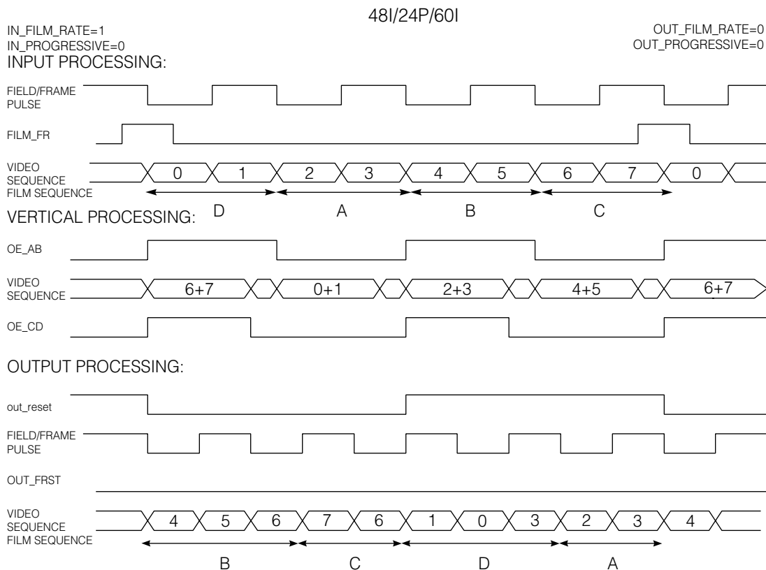
Fig. 30 48I/24P/60I Processing
