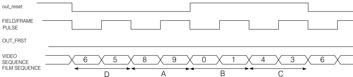
Fig. 18 60I/24P/48I Processing
