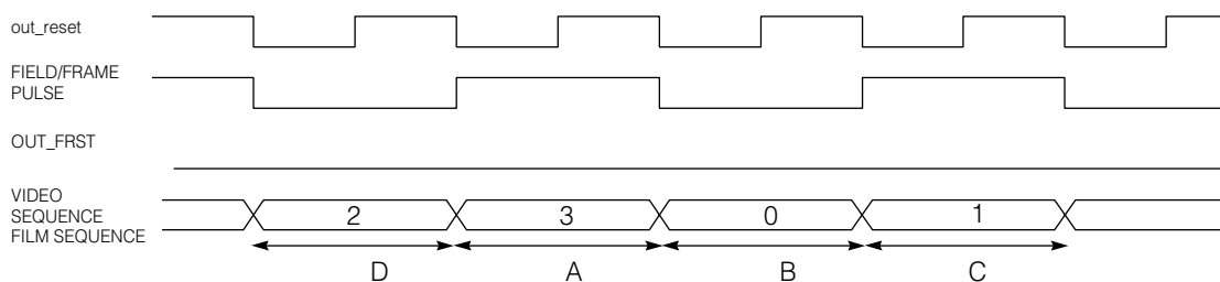
Fig. 40 24P/24P/24P Processing
