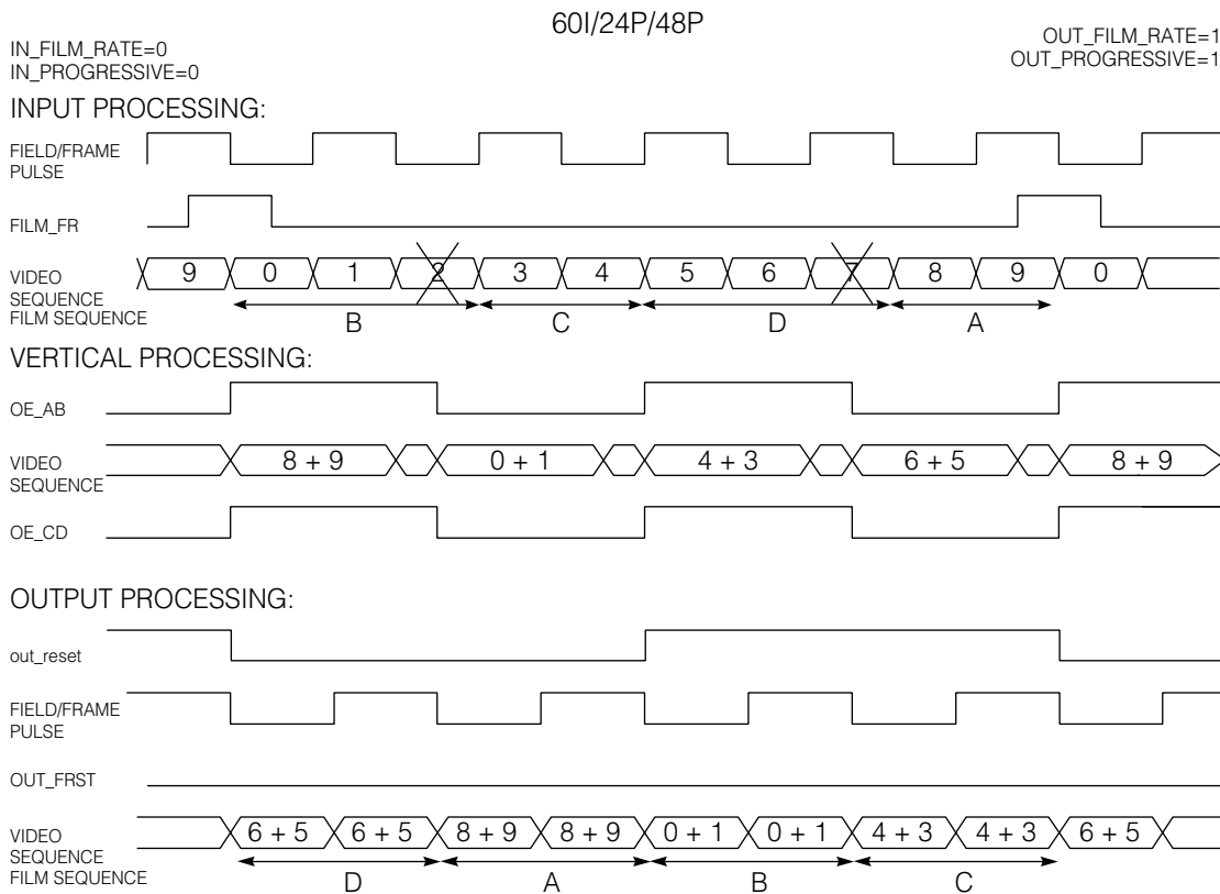
Fig. 23 60I/24P/48P Processing
