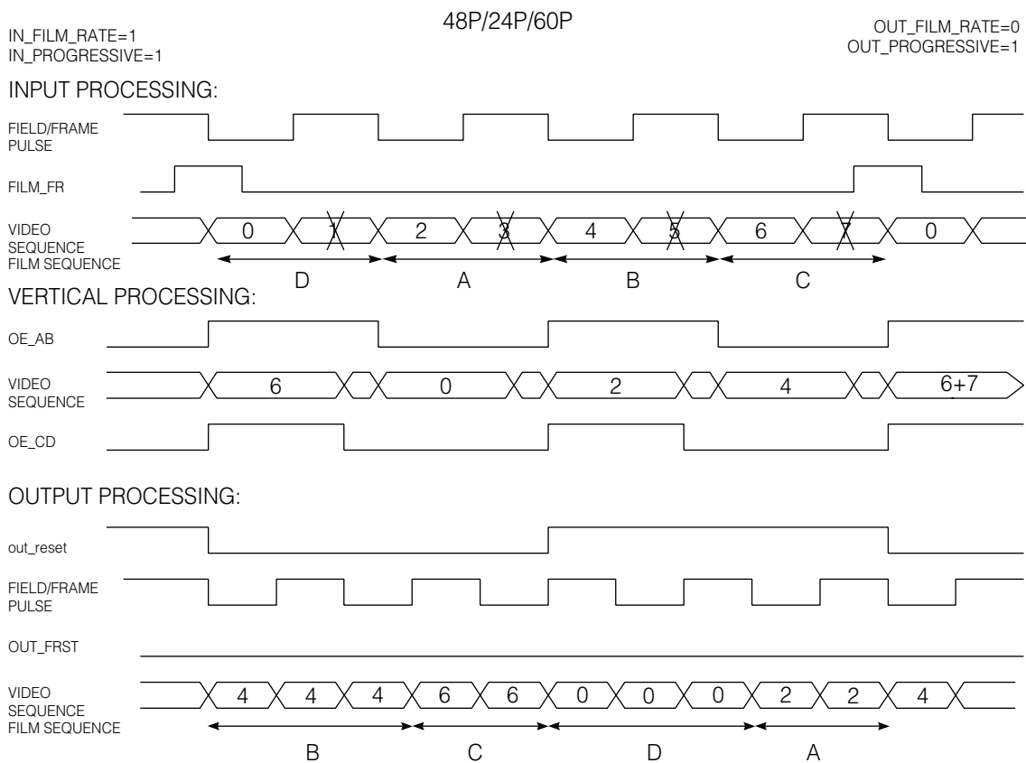
Fig. 32 48P/24P/60P Processing
