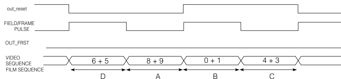
Fig. 20 60I/24P/24P Processing
