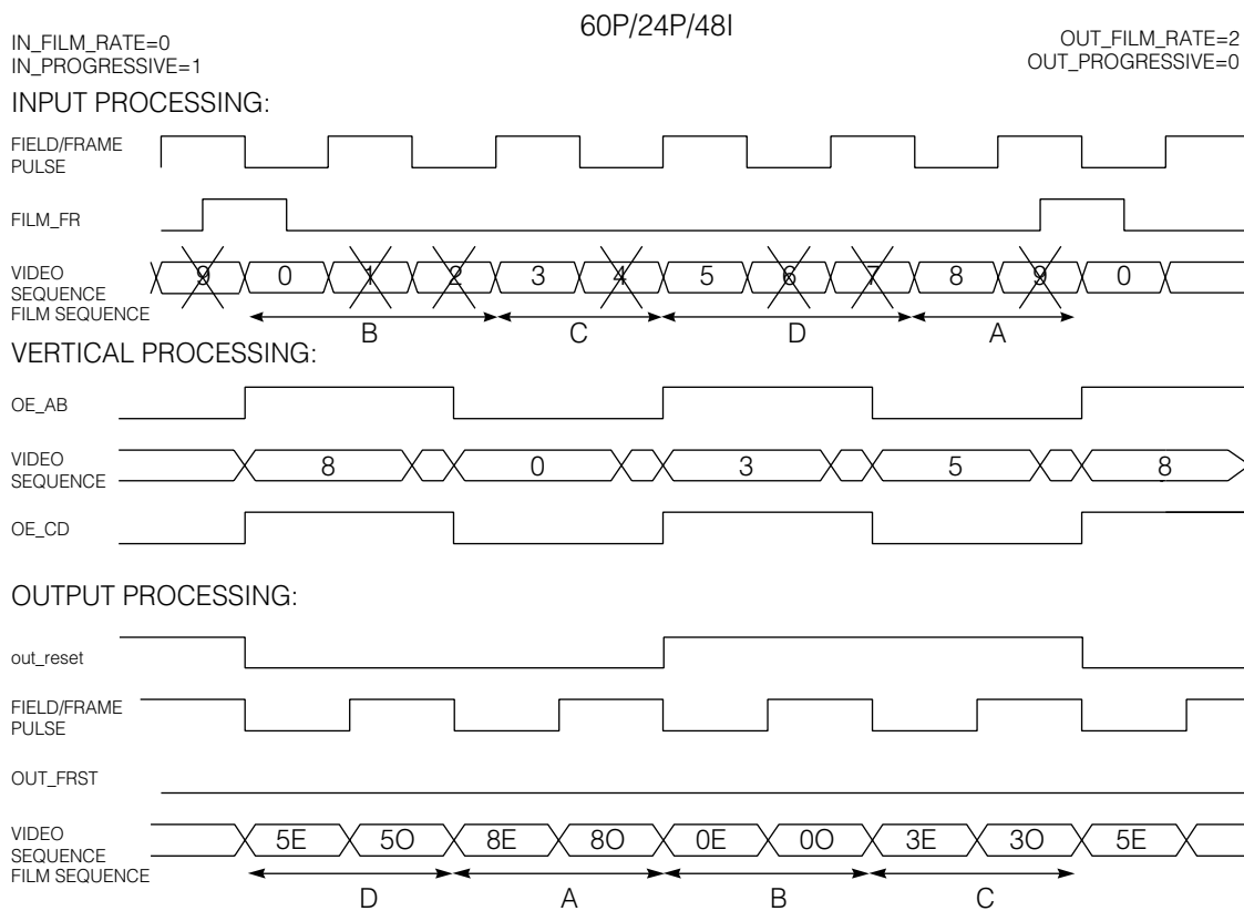
Fig. 25 60P/24P/48I Processing
