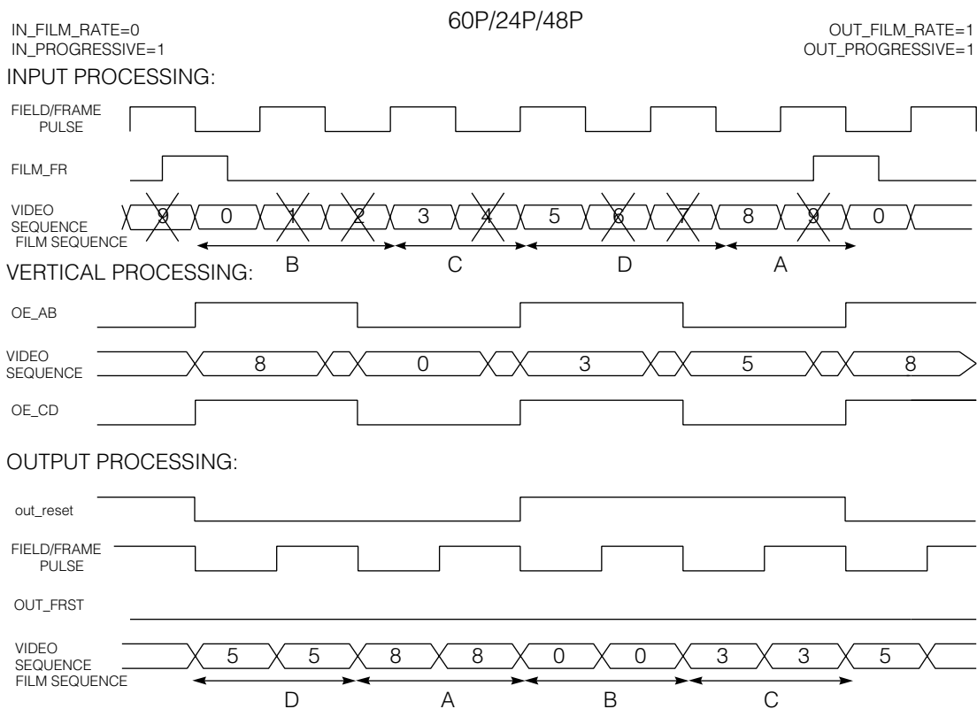
Fig. 24 60P/24P/48P Processing
