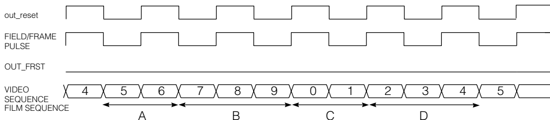
Fig. 21 60P/24P/60I Processing
