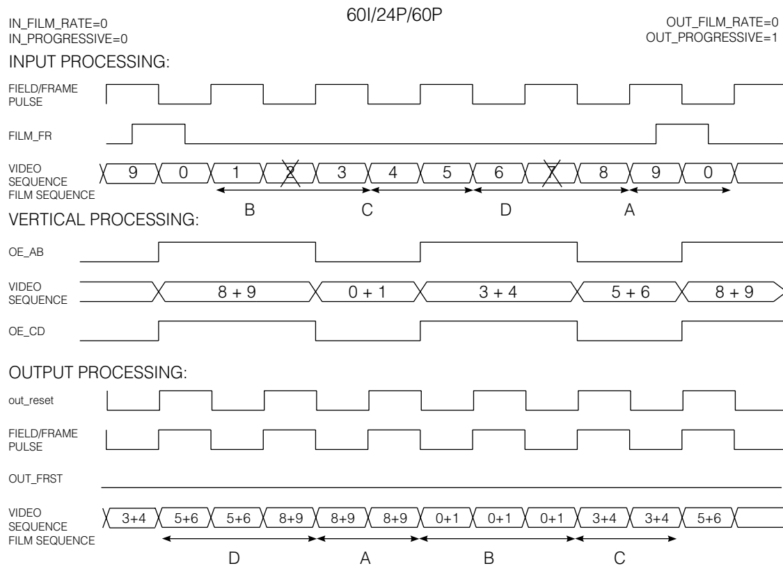
Fig. 29 60I/24P/60P Processing
