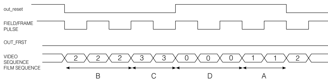
Fig. 41 24P/24P/60P Processing
