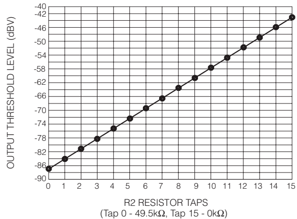
Fig. 14 Threshold Adjustment
