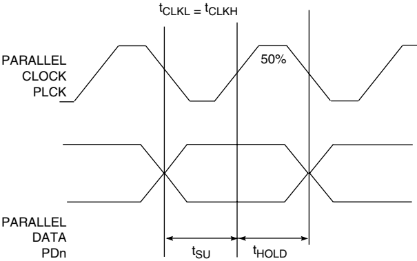
Fig. 4 Waveforms
