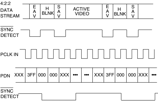
Fig. 5 Timing Diagram
