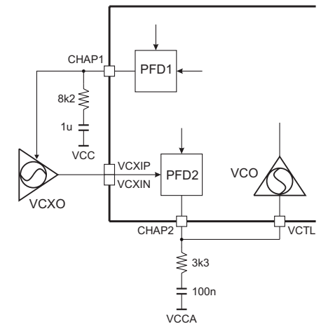
Figure 3. Loop Filters
