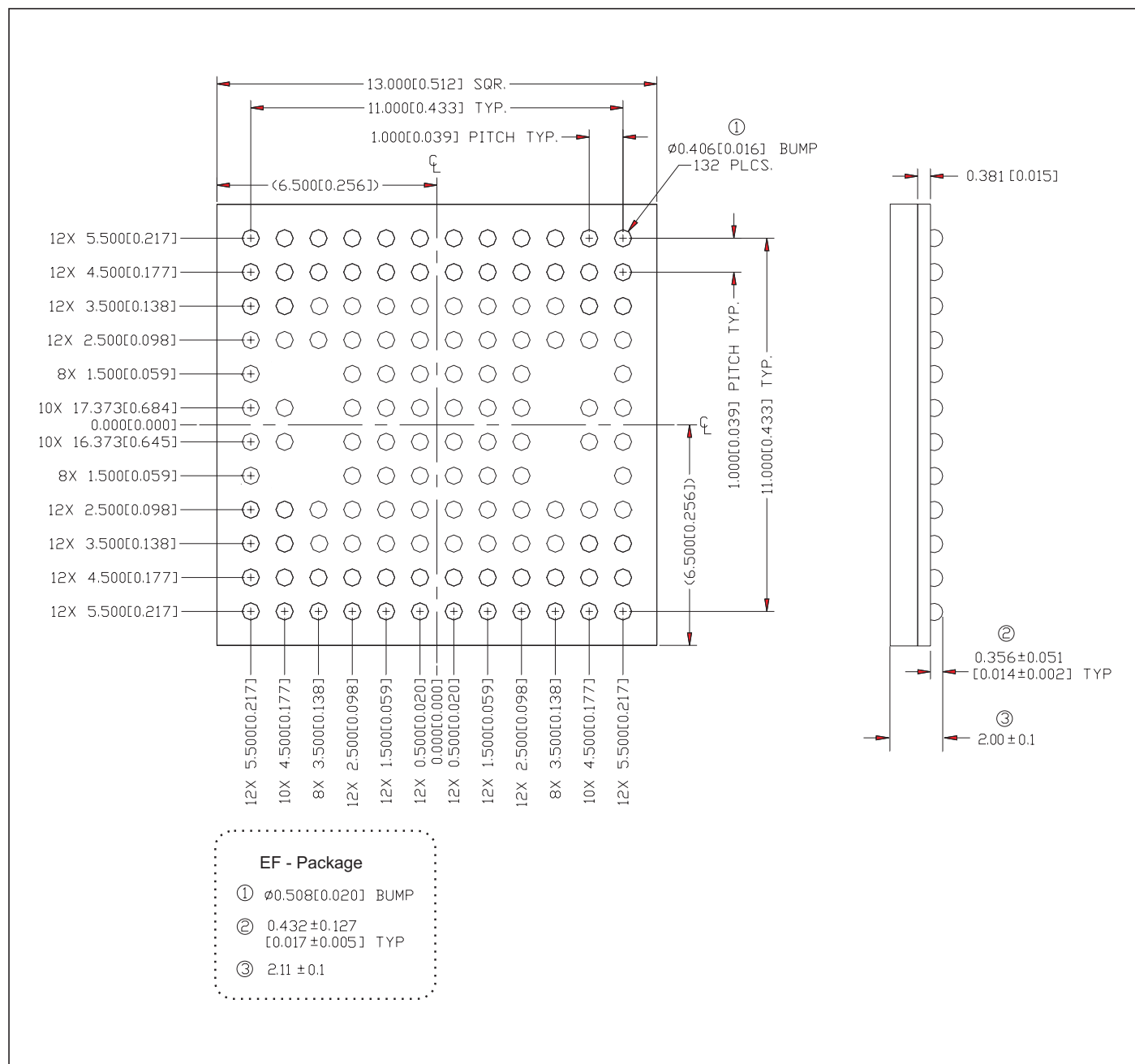
Figure 9. Package 132 ball ceramic BGA (EB package). All dimensions are in mm.
