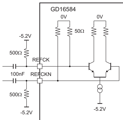
Figure 6. Reference Clock Input (REFCK/REFCKN), Differential AC Coupled.
