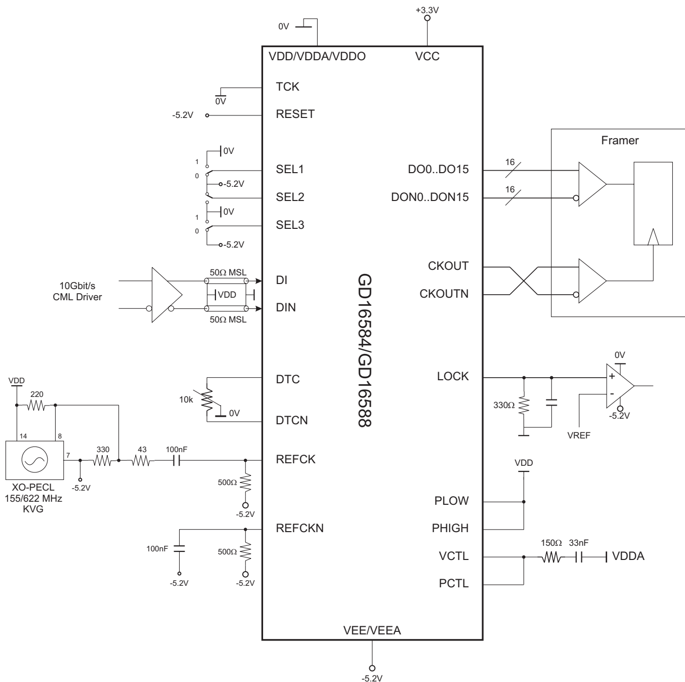
Figure 1. Application Information.
