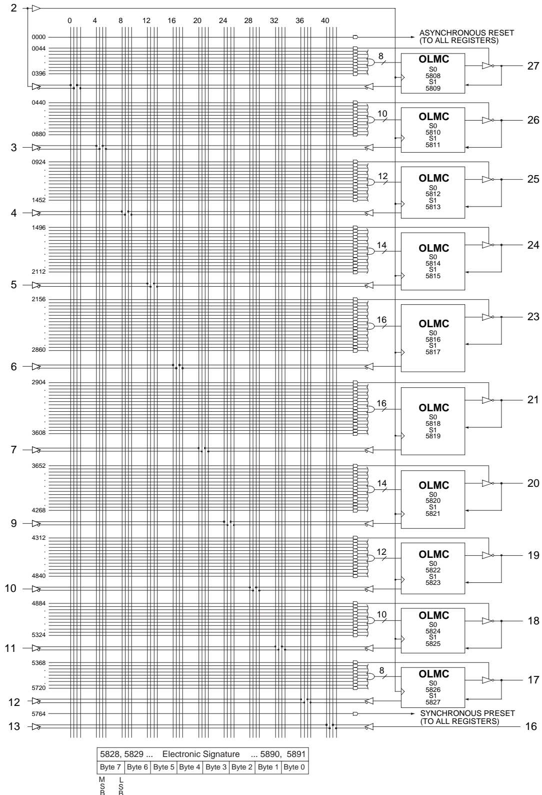
PLCC Package Pinout
