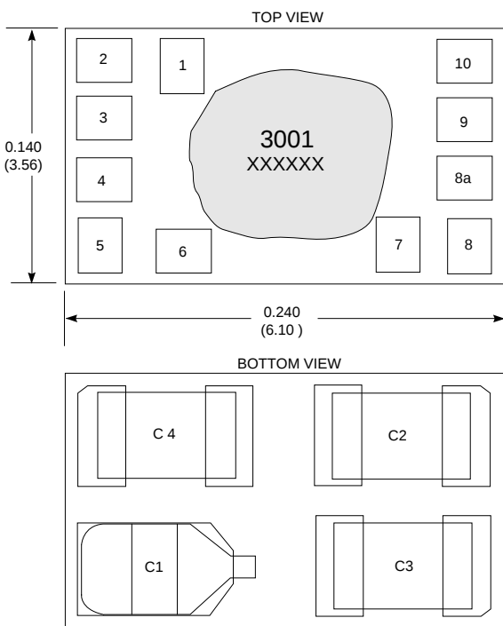
Fig. 10 Hybrid Layout and Dimensions
