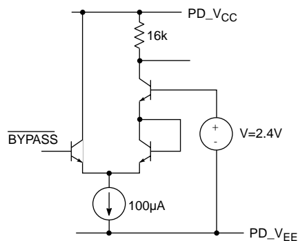
Fig. 11 \overline{\text{BYPASS}} Circuit
