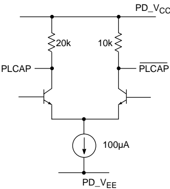
Fig. 4 PLCAP/PLCAP Output
