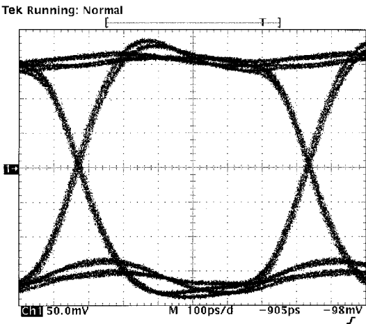
Fig. 21 Uncompensated Output Eye Waveform
