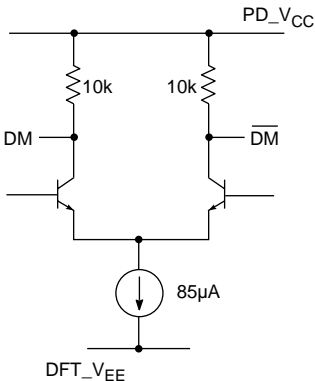
Fig. 3 DM/DM Output
