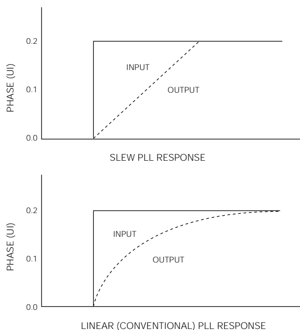
Fig. 13 PLL Characteristics
