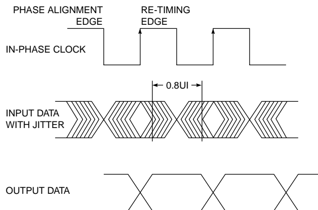
Fig. 14 Phase Detector Characteristics
