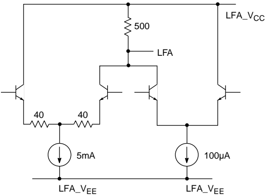
Fig. 5 LFA Circuit
