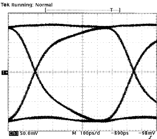
Fig. 22 Compensated Output Eye Waveform
