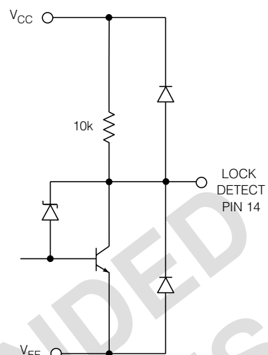
Fig. 2 Lock Detect
