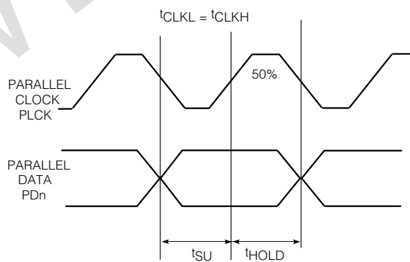
Fig. 4 Input Clock / Data Timing
