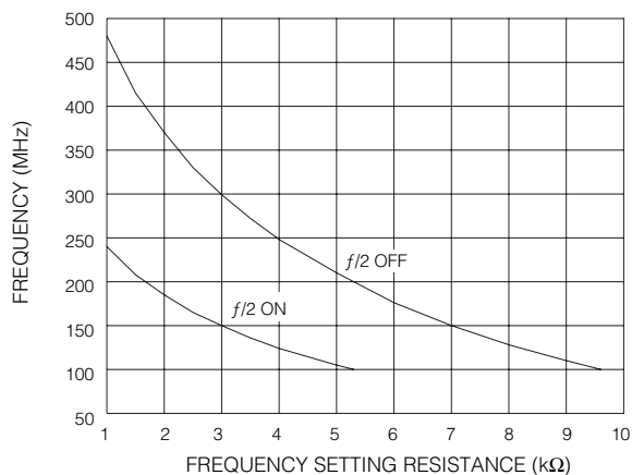
Fig. 9 Clock Frequency
