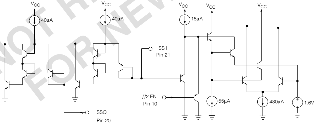
Fig. 8 Pins 20, 21 and 10
