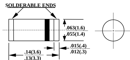
CASE-DO-213AA (GL34) DIMENSIONS IN INCHES AND (MILLIMETERS)
