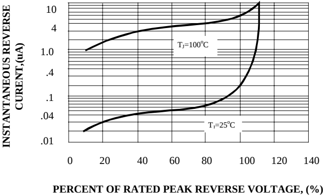
FIG. 4 - TYPICAL REVERSE CHARCETERISTICS
