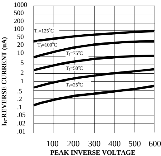
Fig. 6-TYPICAL REVERSE CHARACTERISTIC
