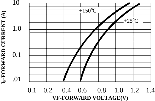
Fig. 4-TYPICAL FORWARD CHARACTERISTICS
