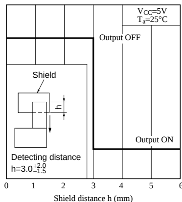
Fig.7 Detecting Position Characteristics (2)
