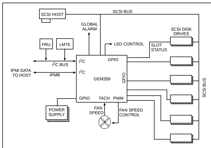
Figure 2. GEM359 SCSI Application
