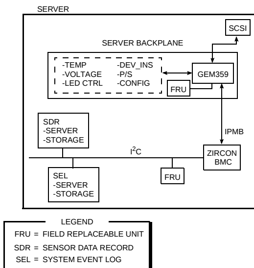
Figure 4. Hot Swap Controller
