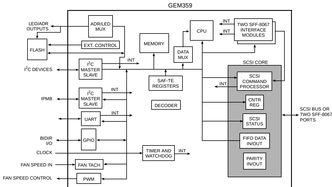
Figure 1. GEM359 Block Diagram
