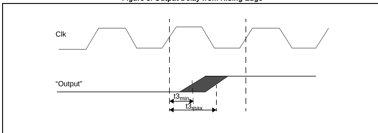
Figure 8: Output Delay from Rising Edge
