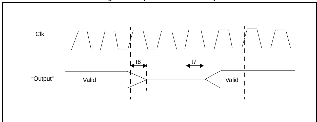
Figure 11: Output Float and Drive Delay
