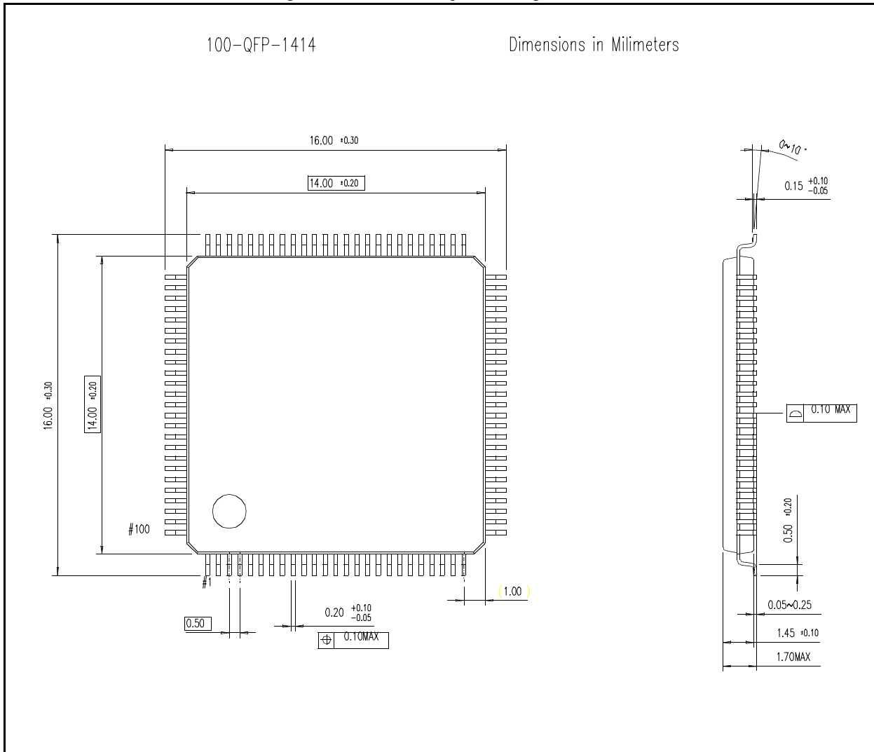
Figure 14: 100 Lead PQFP Package Outline
