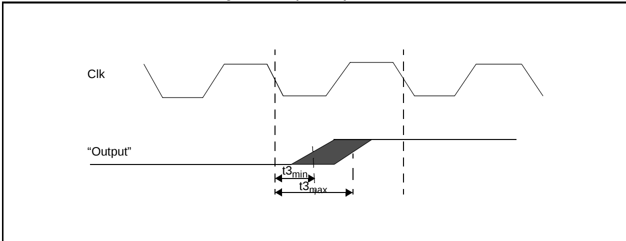
Figure 10: Output Delay from Clock
