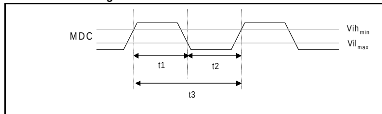
Figure 4: GT-48006A MDC Waveform
