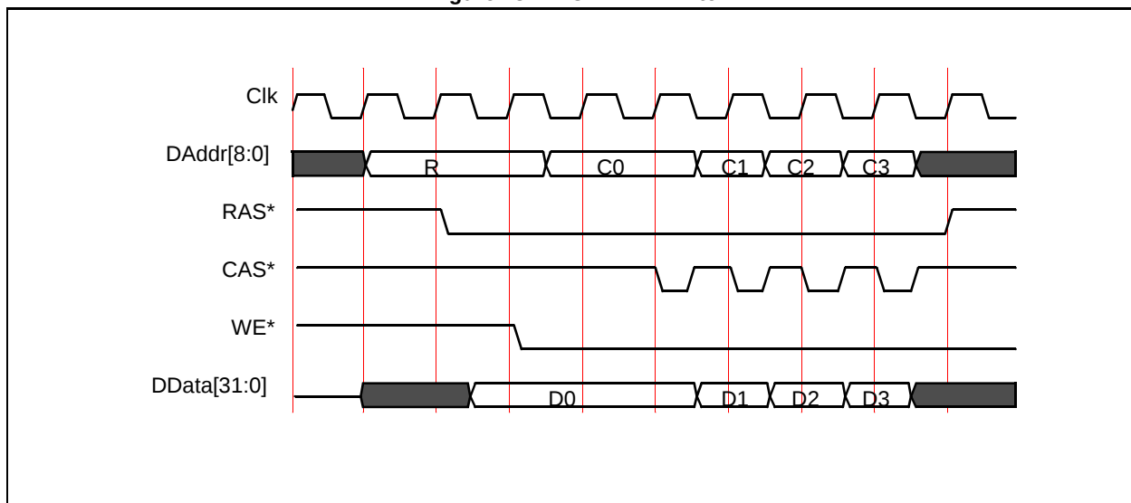
Figure 13: EDO DRAM Write
