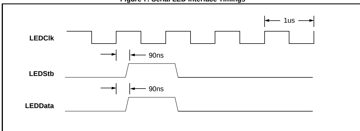
Figure 7: Serial LED Interface Timings
