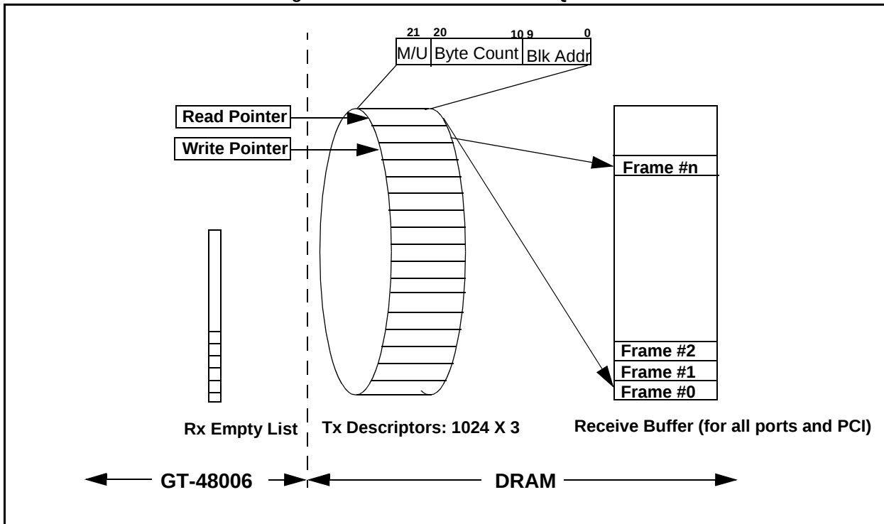
Figure 1: GT-48006A Buffers and Queues
