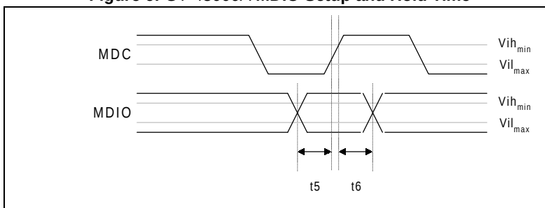
Figure 6: GT-48006A MDIO Setup and Hold Time
