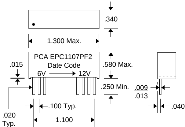
PACKAGE Q
