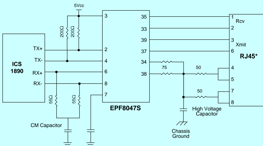
Typical Application Circuit for UTP (only one port shown)
