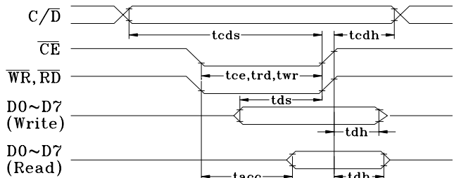
Fig.8-2 Signal timing
