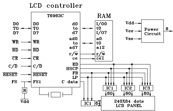
Fig.8-1 Block diagram
