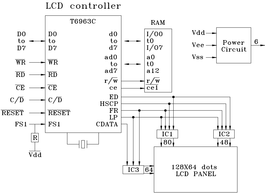
Block diagram
