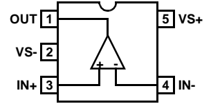
EL5151 (5-PIN SOT-23) TOP VIEW
