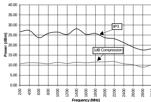
IIP3 &amp; 1dB Compression
