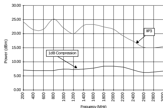
IIP3 & 1dB Compression
