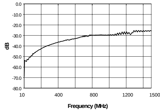
L-R Isolation
