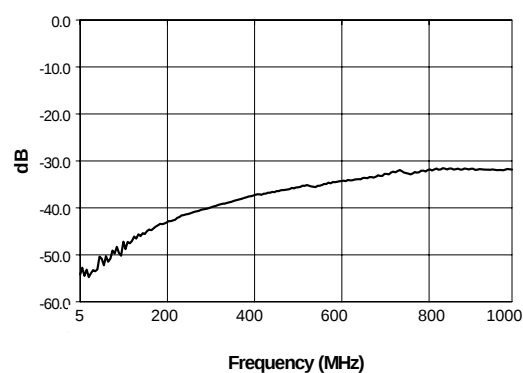
L-R Isolation
