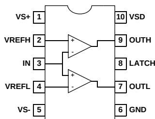
EL5287 (10-PIN MSOP) TOP VIEW
