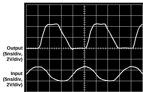
Output with 50MHz Input V_{IN} = 3V_{P-P}
