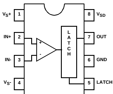
EL5185 (8-PIN SO) TOP VIEW
