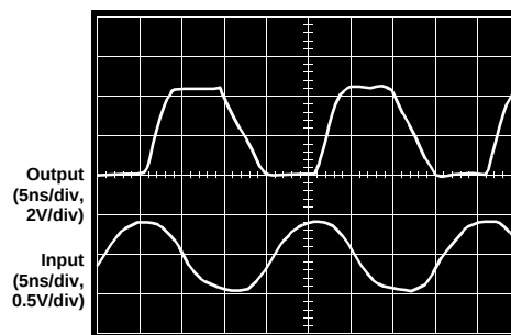
Output with 50MHz Input V_{IN} = 1V_{P-P}
