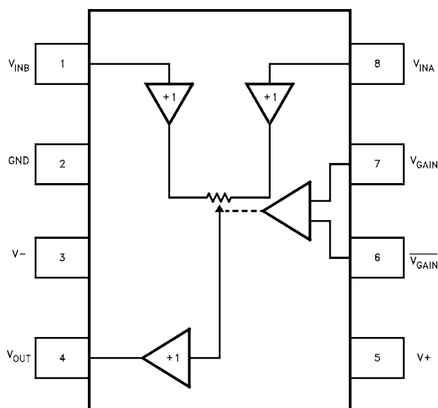
EL4094 (8-PIN PDIP, SO) TOP VIEW
