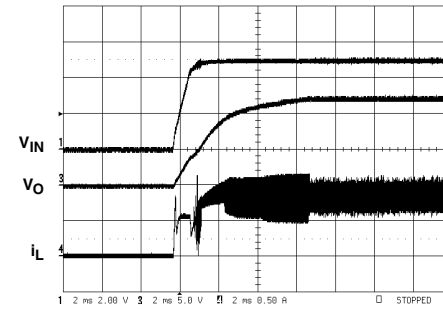
Power-Up V_{IN}=5V , V_O=12V , I_O=300mA
