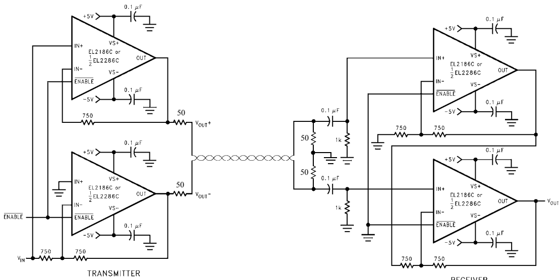
DIFFERENTIAL LINE-DRIVER/RECEIVER
