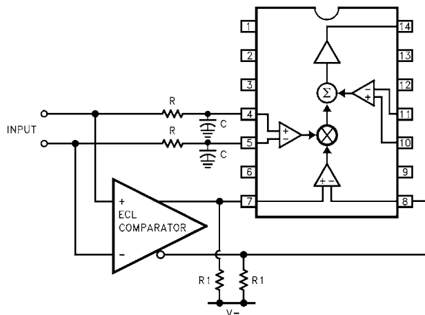
FIGURE 3. ABSOLUTE-VALUE INPUT CIRCUITRY
