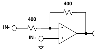
FIGURE 2. A_V = -1
