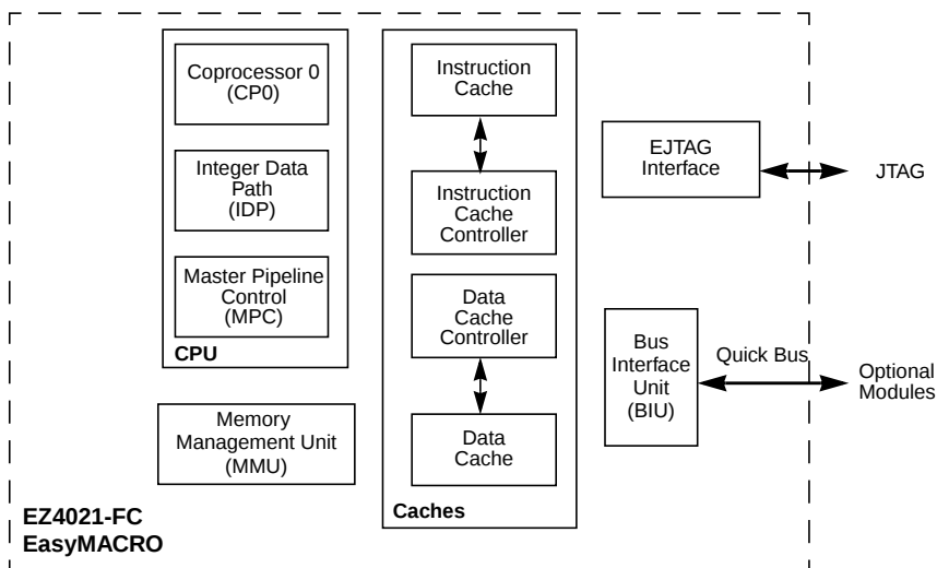
Figure 1 EZ4021-FC Microprocessor EasyMACRO Block Diagram
