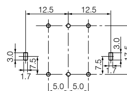
Recommended PWB piercing plan (Top View)
