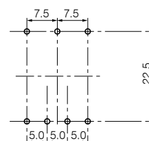
Recommended PWB piercing plan (Top View)
