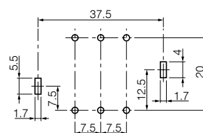
Recommended PWB piercing plan (Top View)
