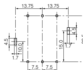
Recommended PWB piercing plan (Top View)
