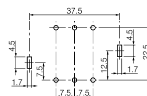
Recommended PWB piercing plan (Top View)
