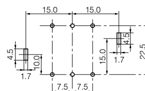
Recommended PWB piercing plan (Top View)
