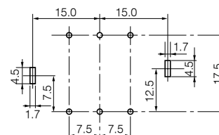
Recommended PWB piercing plan (Top View)
