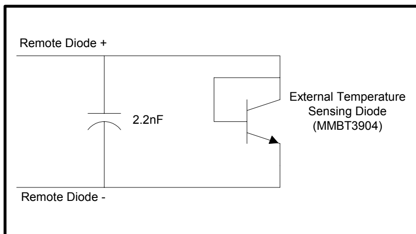
Figure 10.5 Remote Diode (Apply to Remote2 Lines)
