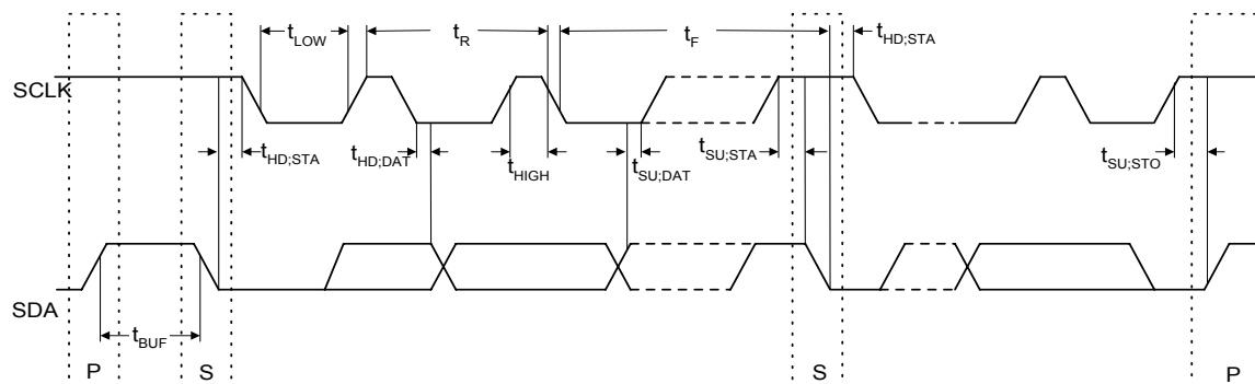
Figure 9.2 SMBus Timing
