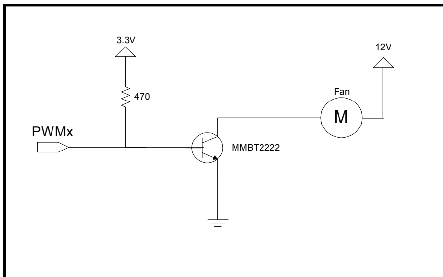
Figure 10.3 Fan Drive Circuitry (Apply to PWM Driving One Fan)
