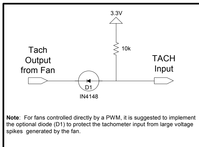
Figure 10.4 Fan Tachometer Circuitry (Apply to Each Fan)
