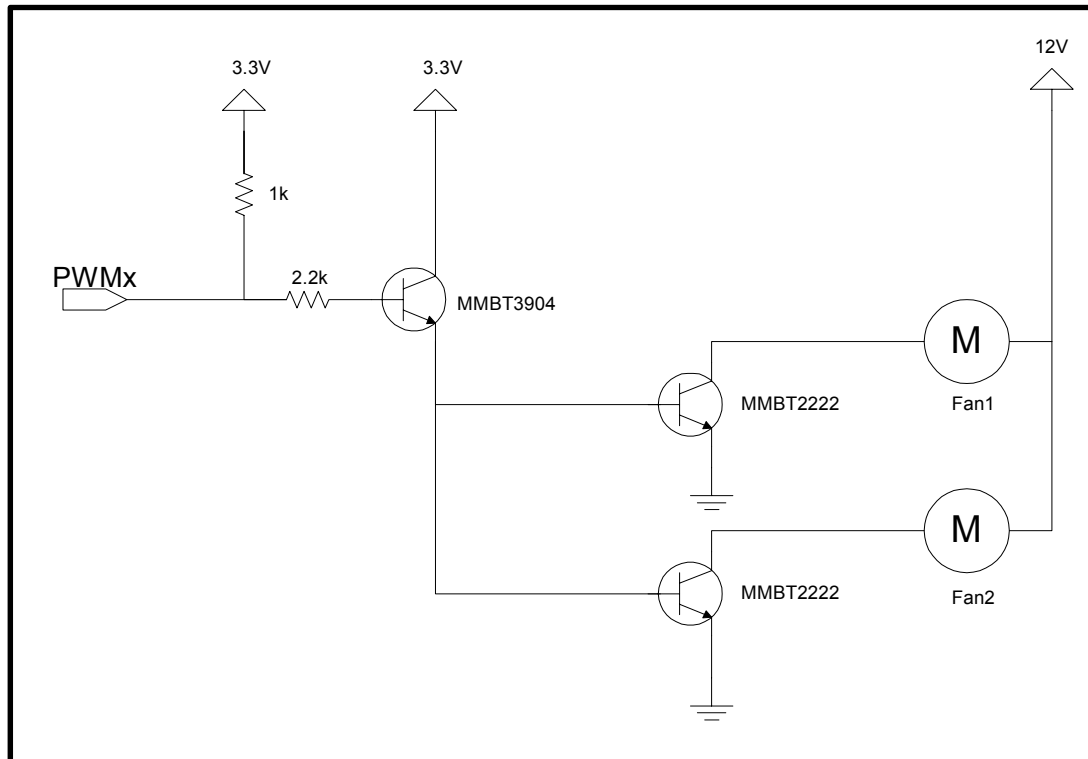
Figure 10.2 Fan Drive Circuitry (Apply to PWM Driving Two Fans)
