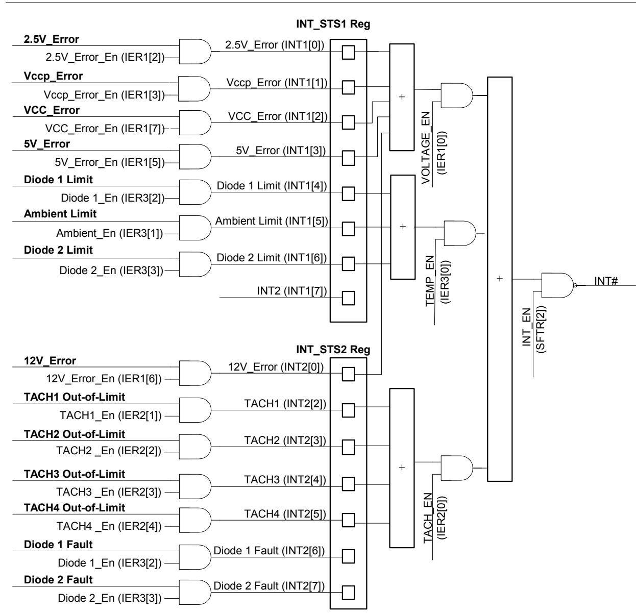
Figure 5.1 Interrupt Control
