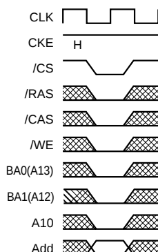
Mode register set command
