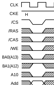
Extended Mode register set command
