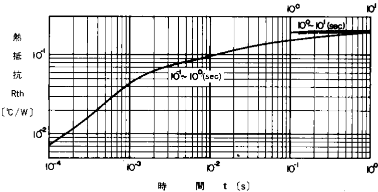
過渡熱抵抗 Transient Thermal Resistance
