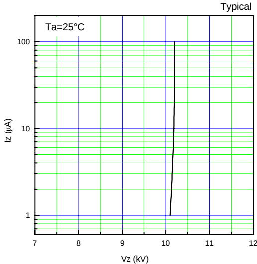
Avalanche characteristic[Vz-Iz]
