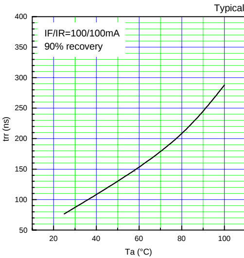
Reverse recovery time characteristic[Ta-trr]
