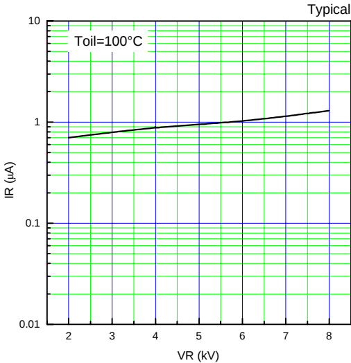
Reverse characteristic[VR-IR]
