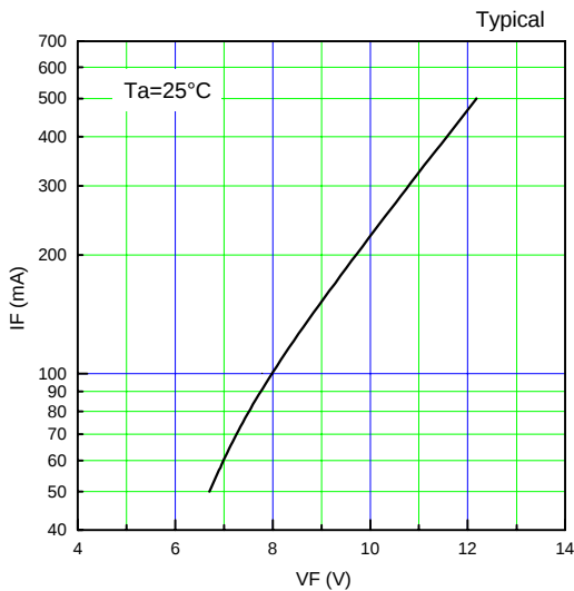
Forward characteistic[VF-IF]
