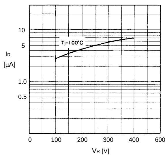
Reverse characteristics
