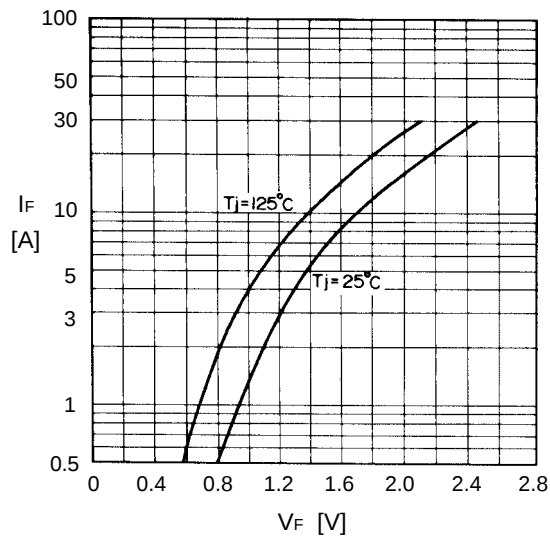
Forward characteristics
