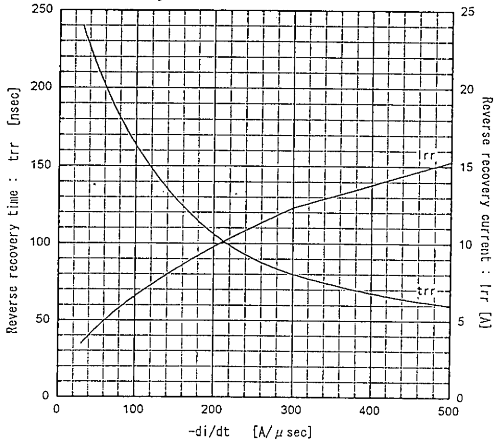
Reverse recovery characteristics vs. -di/dt I_F = 8\text{A} , T_j = 125^\circ\text{C}
