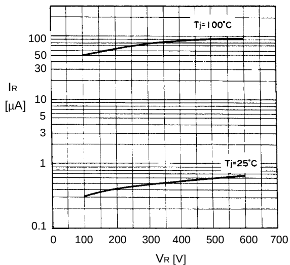
Reverse characteristics
