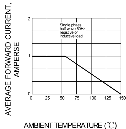
FIG.2 -- TYPICAL FORWARD CURRENT DERATING CURVE
