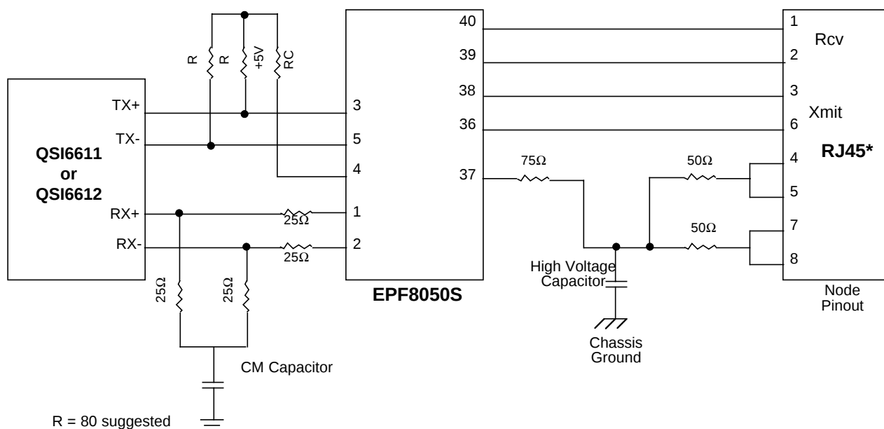
Typical Application Circuit for UTP
