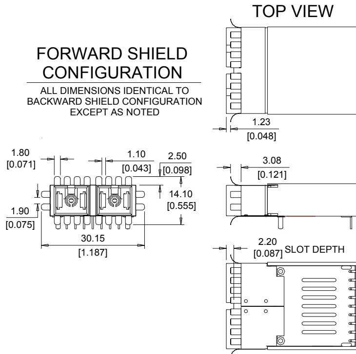
Figure 1B – Forward Shield Transceiver Mechanical Dimensions in mm [inches].
