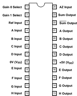
24-Pin QSOP
